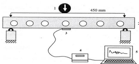
Gambar 2. Set up peralatan uji bending
