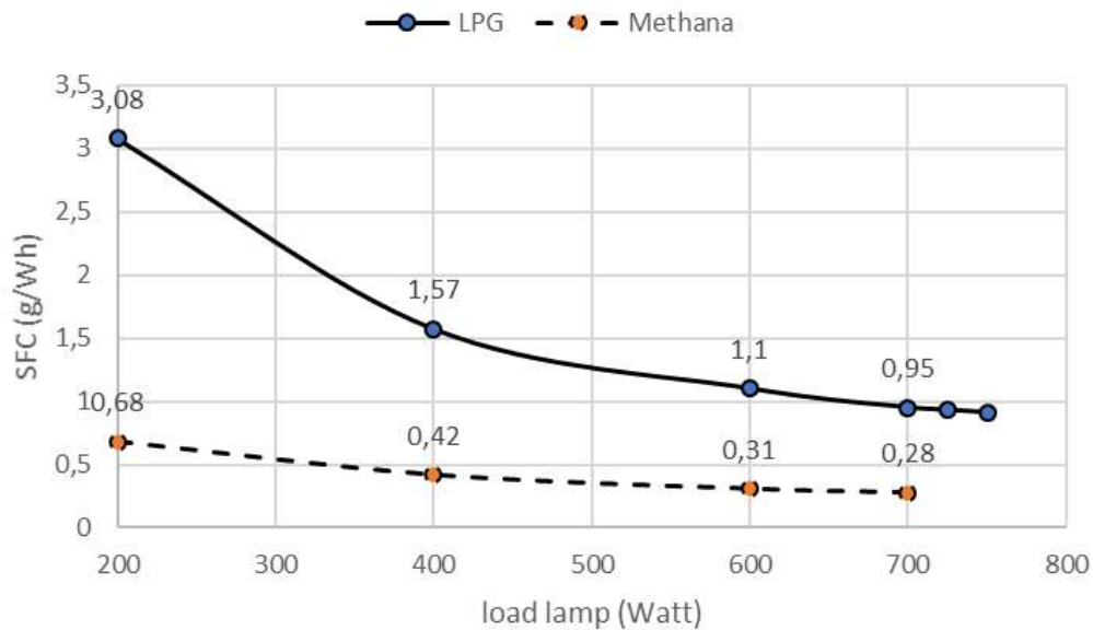
Fig. 3. The value of SFC for various load lamp.
