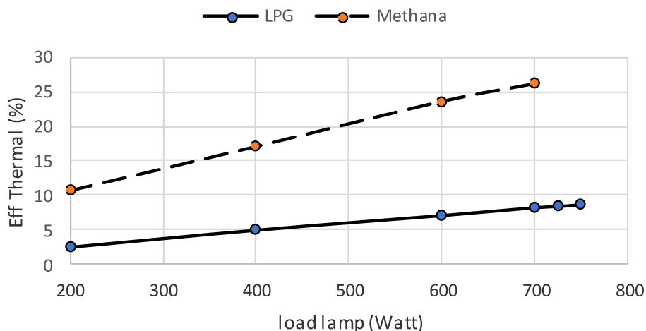
Fig. 4. Thermal Efficiencies of genset with methana and LPG as fuel
