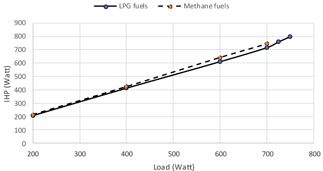
Fig. 2. The value of IHP for various lamp load on the generator.
