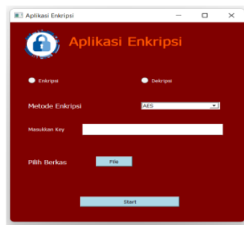
Figure 2. Encryption tools.
