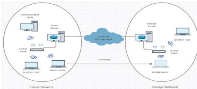
Gambar 1. Network topology.
