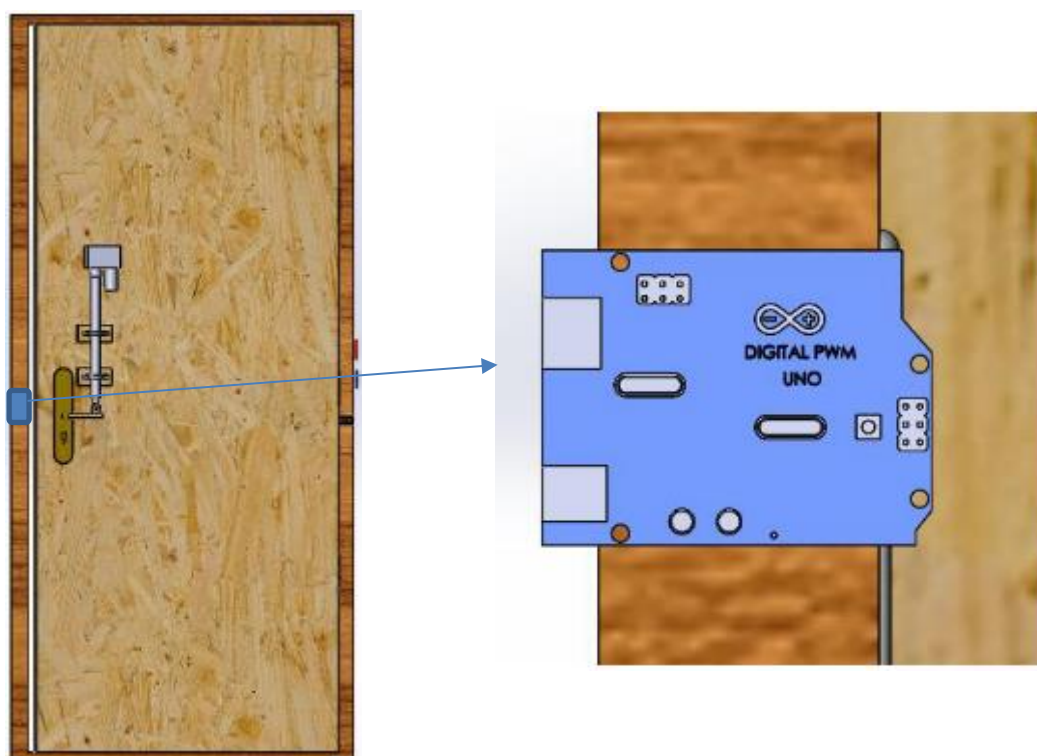
Figure 3. Location of the sensor and actuator motor.
