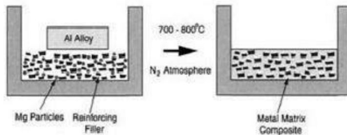
Figure 1. Scheme of process infiltration of composite materials based on canned waste
