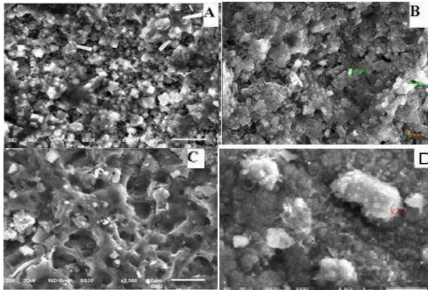
Figure 4. SEM results of composite with (a) 20 vol.% Al 2 O 3 : 14 vol.% Mg with 2000x magnification, (b) 20 vol.% Al 2 O 3 : 15 vol.% Mg with 5000x magnification, (c) 10 vol.% Al 2 O 3 : 15 vol.% Mg with 2000x magnification, (d) 10 vol.% Al 2 O 3 : 16 vol.% Mg with 5000x magnification
