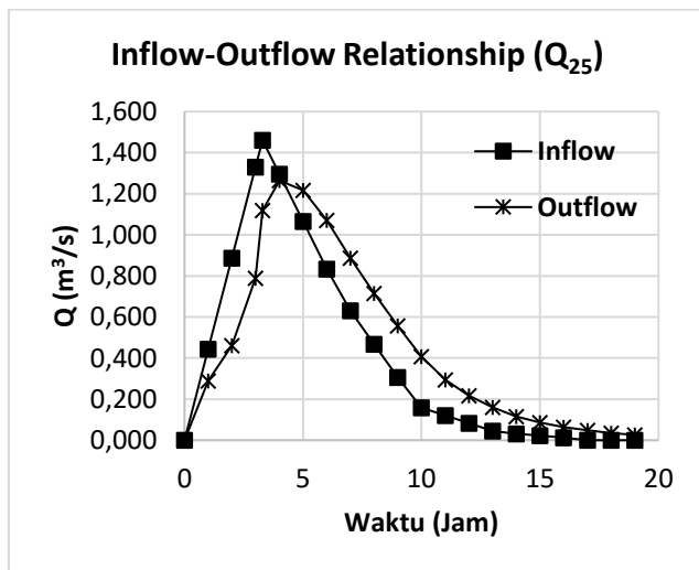
Gambar 9. Inflow-Outflow Relationship ( Q_{25} ) Sumber: Hasil Analisis
