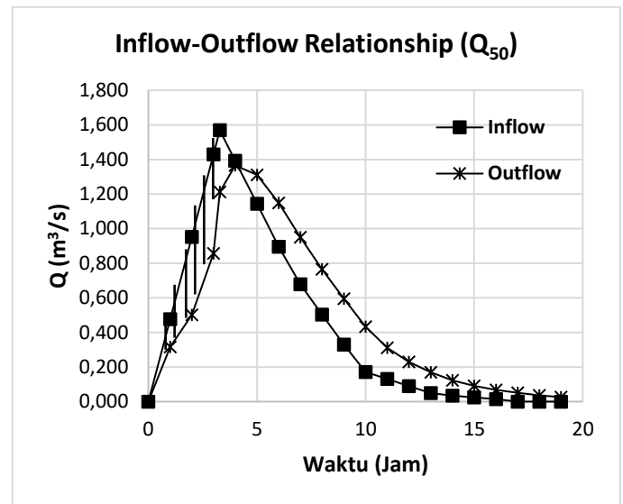
Gambar 10. Inflow-Outflow Relationship ( Q_{50} ) Sumber: Hasil Analisis
