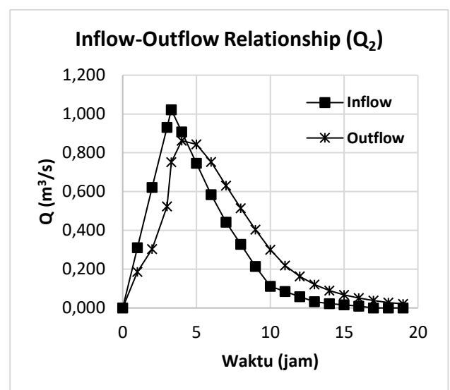
Gambar 8. Inflow-Outflow Relationship ( Q_2 ) Sumber: Hasil Analisis
