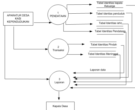
Gambar 2. Data Flow Diagram (DFD) level 0
