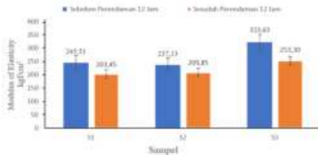
Gambar 4.6 Hasil Modulus of Elasticity
