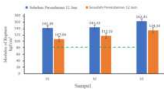
Gambar 4.7 Hasil Modulus of Rupture
