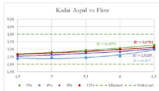
Gambar 5.21 Grafik perbandingan kadar aspal vs flow
