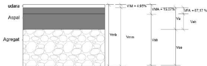
Gambar 5.15 Contoh skematis rongga beton aspal padat kadar aspal 6% AAT 4%
