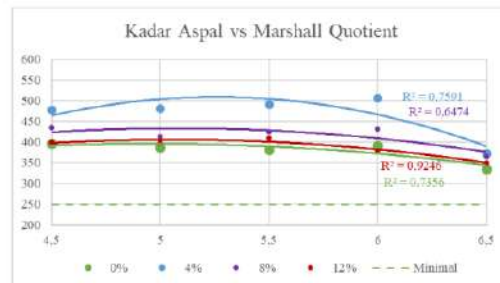
Gambar 5.22 Grafik perbandingan kadar aspal vs marshall quotient
