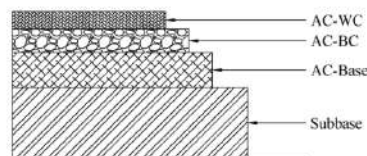
Gambar 3.3 Lapis aspal beton
