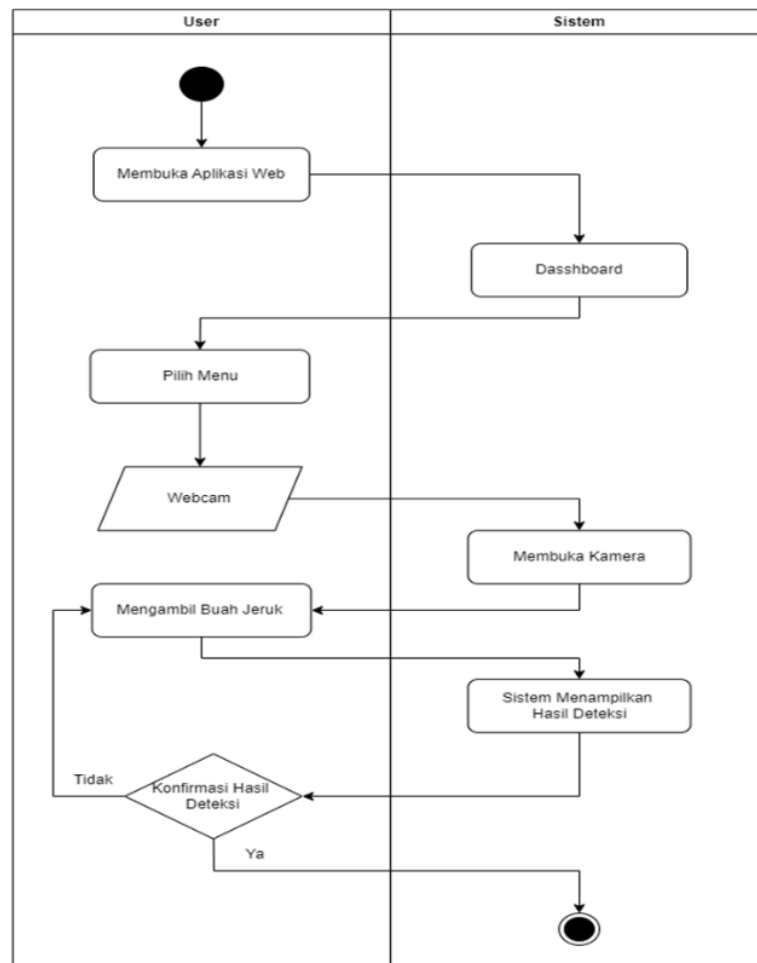
Gambar 3.6 Activity Diagram Webcam
