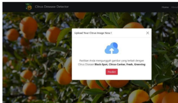
Gambar 4.11 Image Detection
