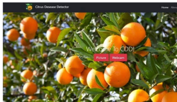
Gambar 4.10 Tampilan Dashboard
