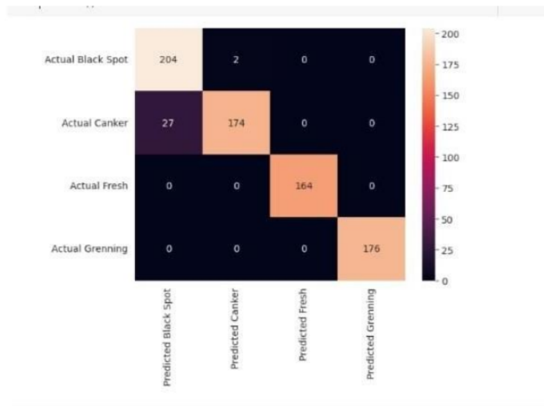
Gambar 4.7 Confussion Matrix Model Mobilenet V2
