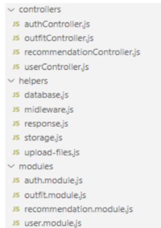
Gambar 3.4 Struktur Folder Program API
