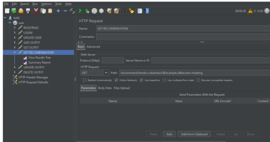
Gambar B. 7 Pengujian Get Recommendation
