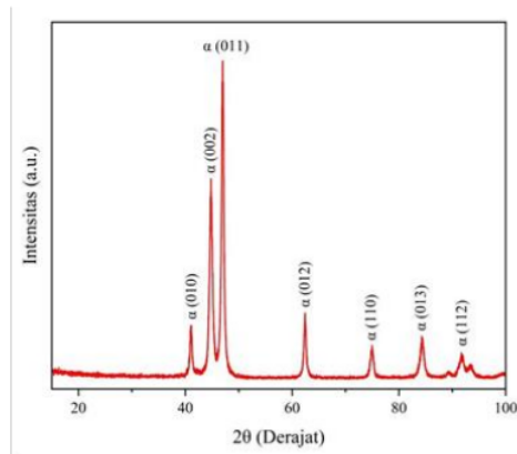
Gambar 4.5 Data XRD Sampel As-Cast Paduan Ti-6Al-5Nb-3Sn-1Zr-0,5Si
