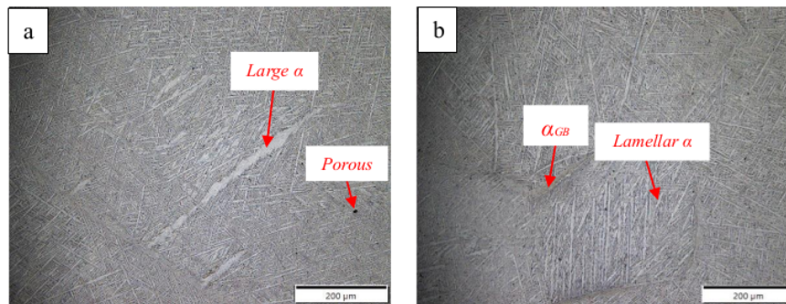
Gambar 4.1 Struktur Mikro As-Cast Paduan Ti-6Al-5Nb-3Sn-1Zr-0,5Si
