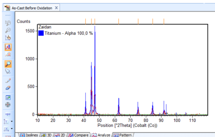
Gambar B.5 Data XRD Paduan As-Cast
