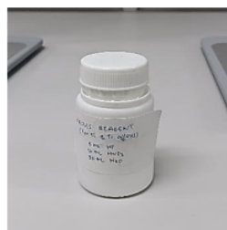
Gambar C.16 Larutan Kroll
