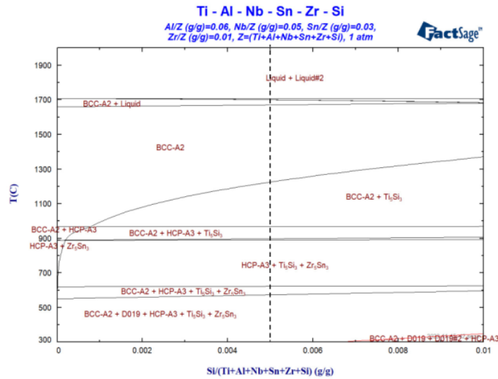
1 Gambar 2.16 Diagram Fasa Ti-6Al-5Nb-3Sn-1Zr-0,5Si ( FactSage )
