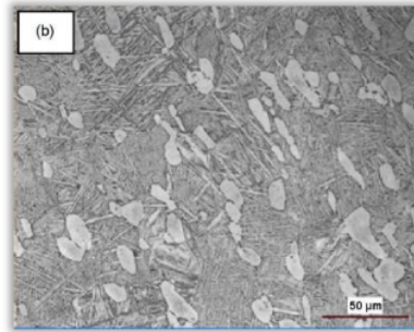
Gambar 2.9 Struktur Mikro Hasil Aging Treatment [41].
