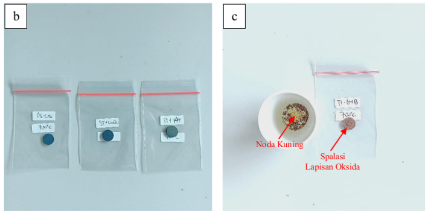
Gambar 4.11 Sampel Pengujian Oksidasi. (a) Sampel Sebelum Pengujian Oksidasi, (b) – (c) Sampel Setelah Pengujian Oksidasi 700°C. (b) Ti-6Al-5Nb-3Sn-1Zr-0,5Si as-cast, solution treatment, aging treatment , (c) Ti-6Al-4V
