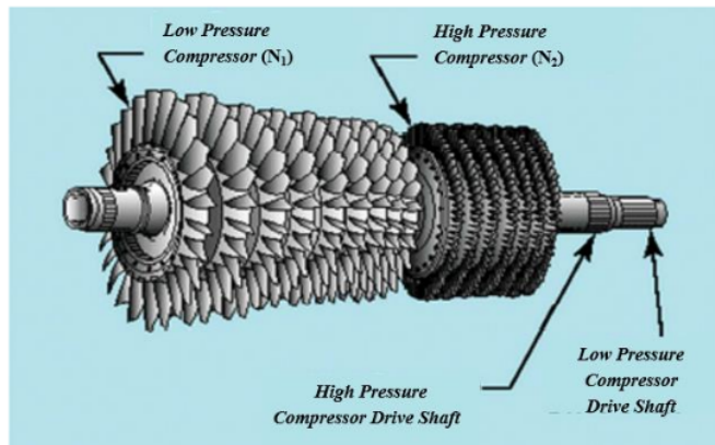
Gambar 2.5 Compressor in Turbine Jet Engine [3].
