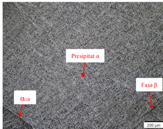
Gambar 4.3 Struktur Mikro Paduan Ti-6Al-5Nb-3Sn-1Zr-0,5Si Aging Treatment
