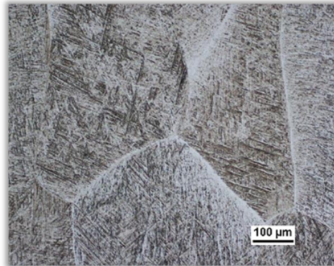
Gambar 2.7 Struktur Mikro Hasil Solution Treatment + Quenching [39].
