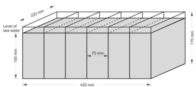
Fig 3. Experiment tank
