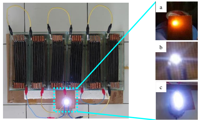
Fig 9. Six cells battery in series connection drive LED. (a) Yellow DIP LED, (b) single high power LED (1 watt), (c) five high power LEDs.
