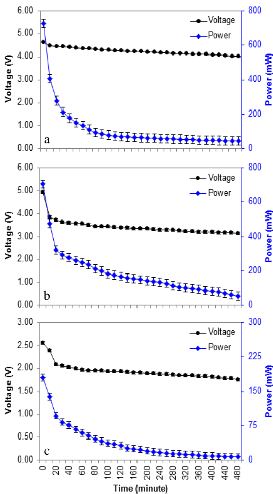
Fig 8. Comparison of voltage and power output of galvalume battery (a), zinc battery (b), aluminium battery (c). Vertical bar denote standard error.
