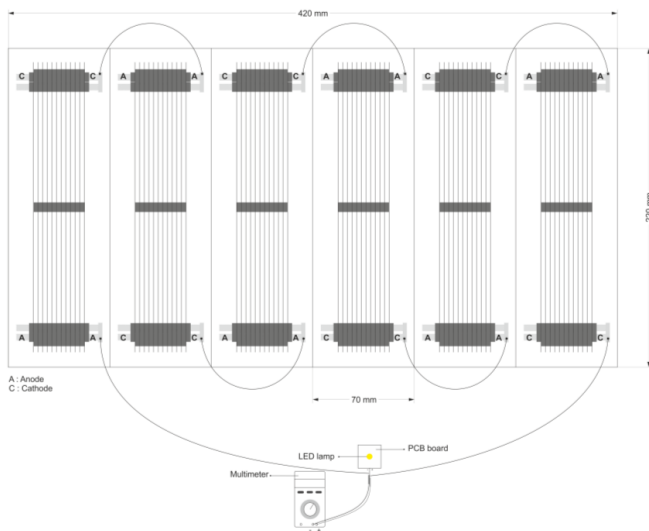
Fig 4. The experiment set-up of load condition
