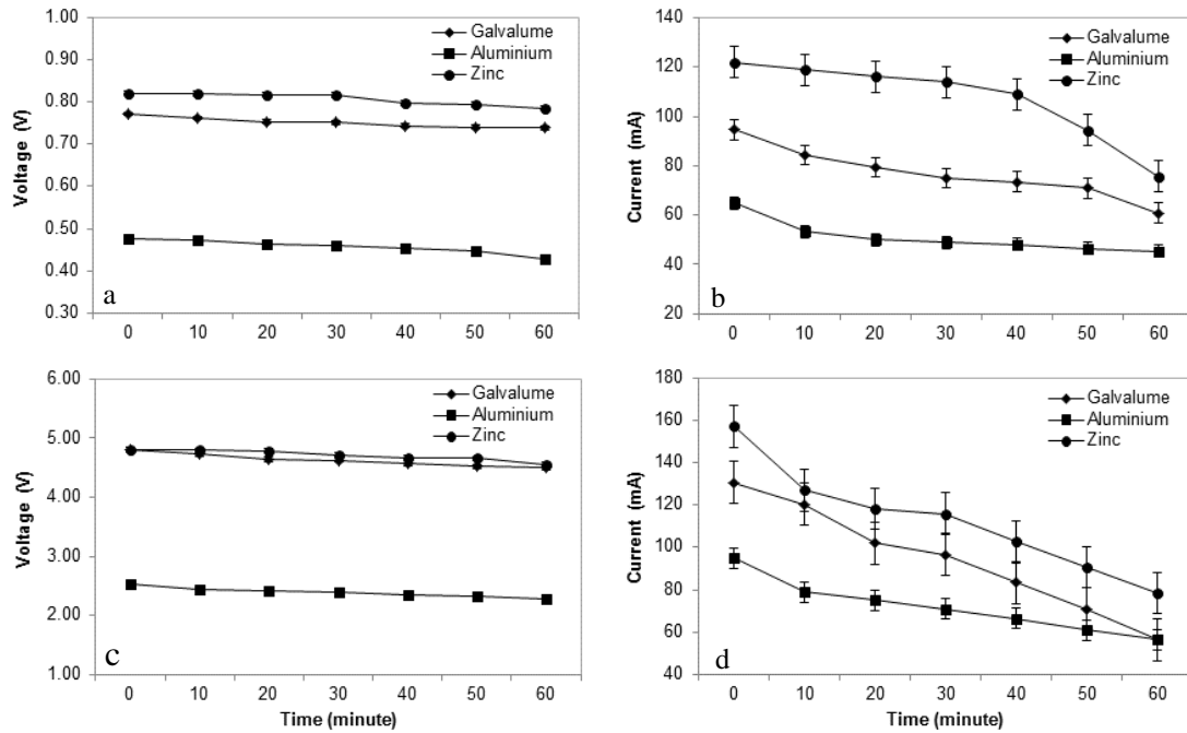
Fig 5. The voltage and current profiles based on time elapsed observation. Single cell battery (a-b). Six cells battery (c-d). Vertical bar denote standard error.
