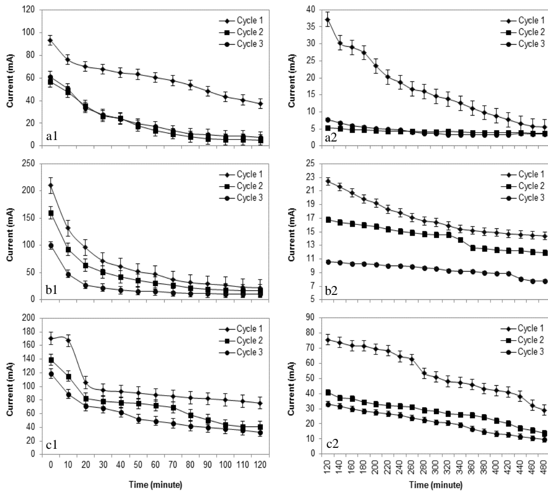
Fig 7. Current profiles of aluminium battery (a1-a2), galvalume battery (b1-b2), zinc battery (c1-c2) based on time elapsed observation. Vertical bar denote standard error.
