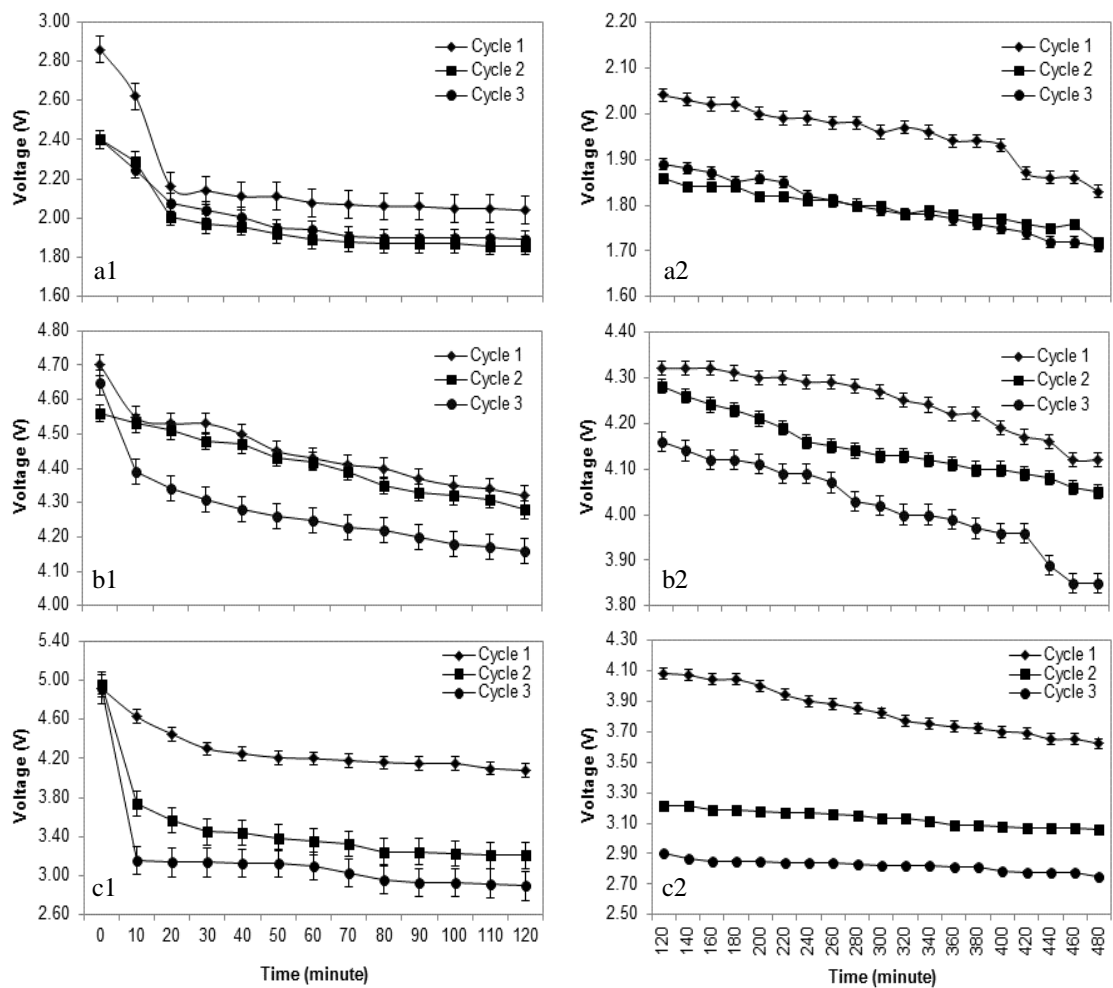
Fig 6. Voltage profiles of aluminium battery (a1-a2), galvalume battery (b1-b2), zinc battery (c1-c2) based on time elapsed observation. Vertical bar denote standard error.
