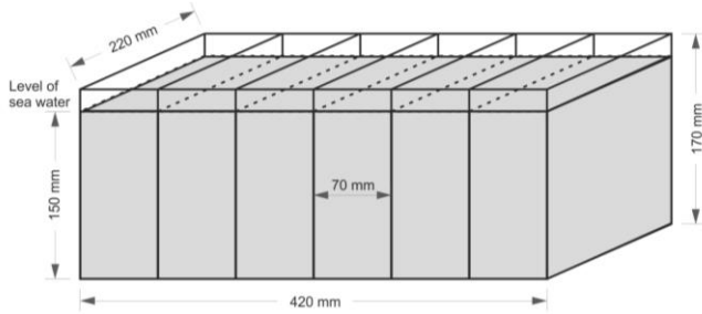
Fig 3. Experiment tank
