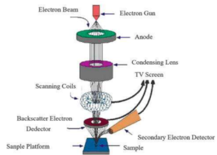
Gambar 2.9 Scanning Electron Microscope (Sumber: intechopen.com)
