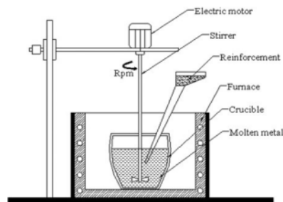
Gambar 2.4 Proses Stir Casting
