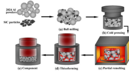
Gambar 2.3 Proses Thixoforming
