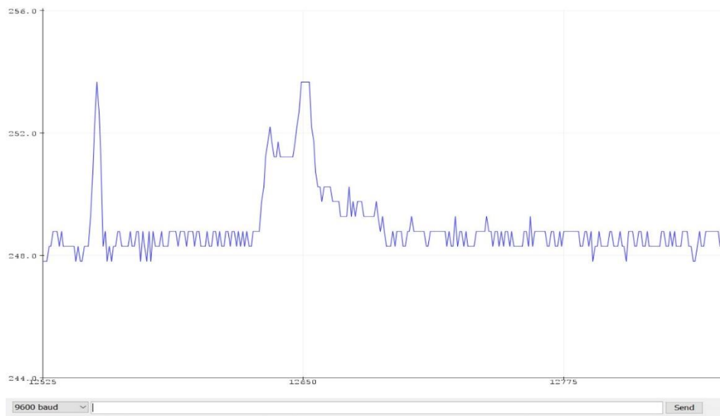
Gambar 3 Pengujian sample 5 Ampere
