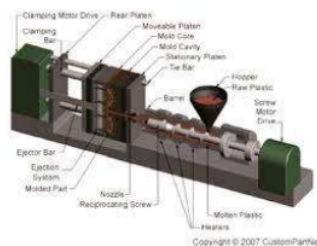
Gambar 2.10 Injection molding (Sumber : www.custompartnet.com )
