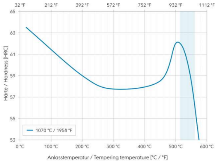
Gambar 3.14 Thempering Chart
