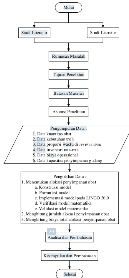
Gambar 4. Flowchart Penelitian
