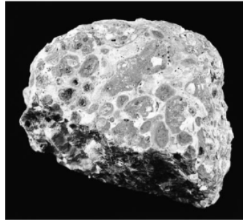
Gambar 2.2 Bijih Bauksit [21]
