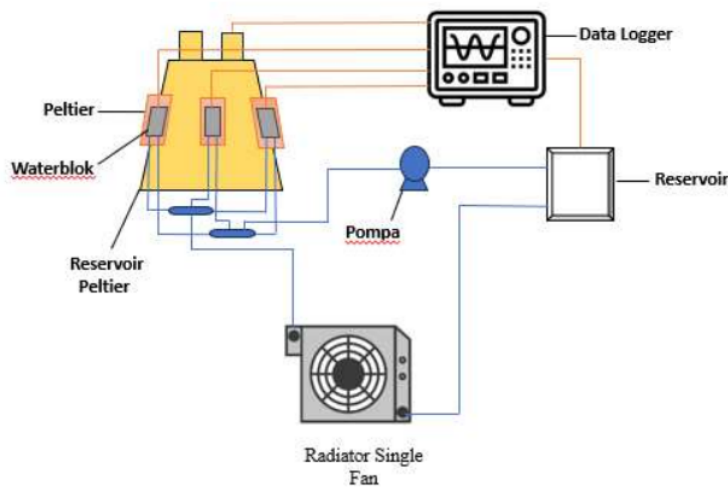
Gambar 3.2 Metode Radiator Single
