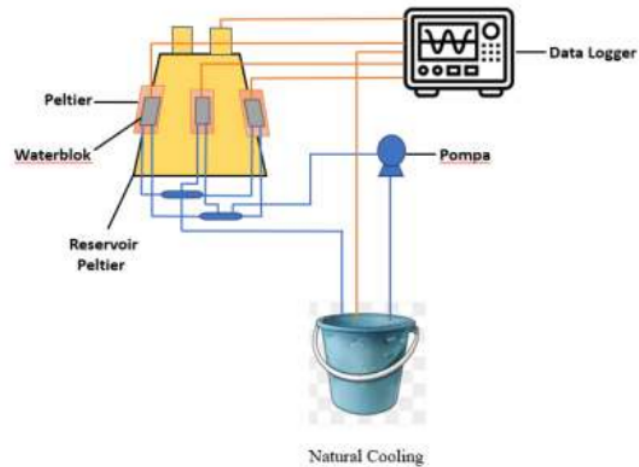
Gambar 3.1 Metode Natural Cooling
