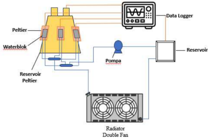
Gambar 3.3 Metode Radiator Double
