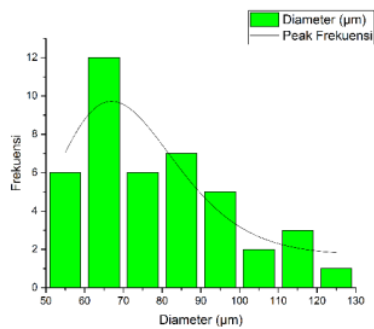
Gambar 4.14 Histogram SEM PUR-11
