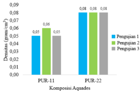
Gambar B.7 Densitas PUR-11 & PUR-22
