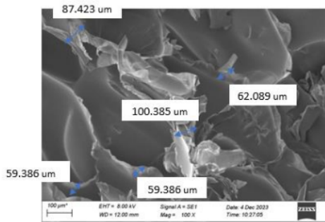
Gambar B.13 SEM PUR-11 Ukuran 100x
