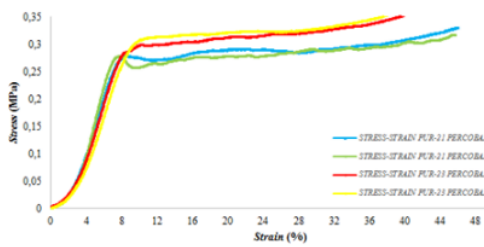
Gambar B.3 Kuat Tekan PUR-21 & 23
