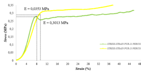
Gambar B.4 Kuat Tekan PUR-21 & 23
