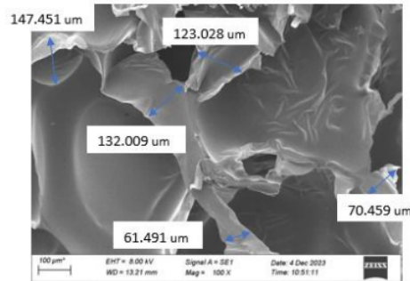
Gambar B.14 SEM PUR-21 Ukuran 100x
