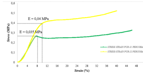
Gambar B.2 Kuat Tekan PUR-11 & PUR-22
