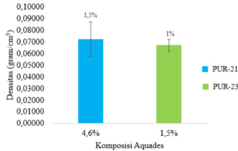
Gambar B.6 Densitas PUR-21 & PUR-23
