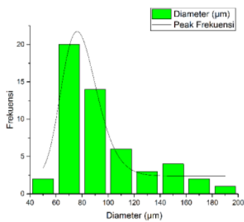
Gambar 4.16 Histogram SEM PUR-22
