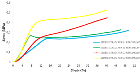
Gambar B.1 Kuat Tekan PUR-11 & PUR-22
