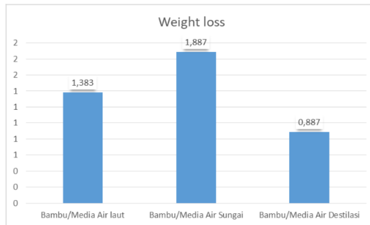
Gambar 4. 6 Grafik Weight Loss Uji TGA
