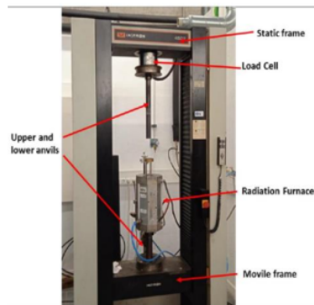
Gambar C.3 Test Machine Hot Compression and Tensile
