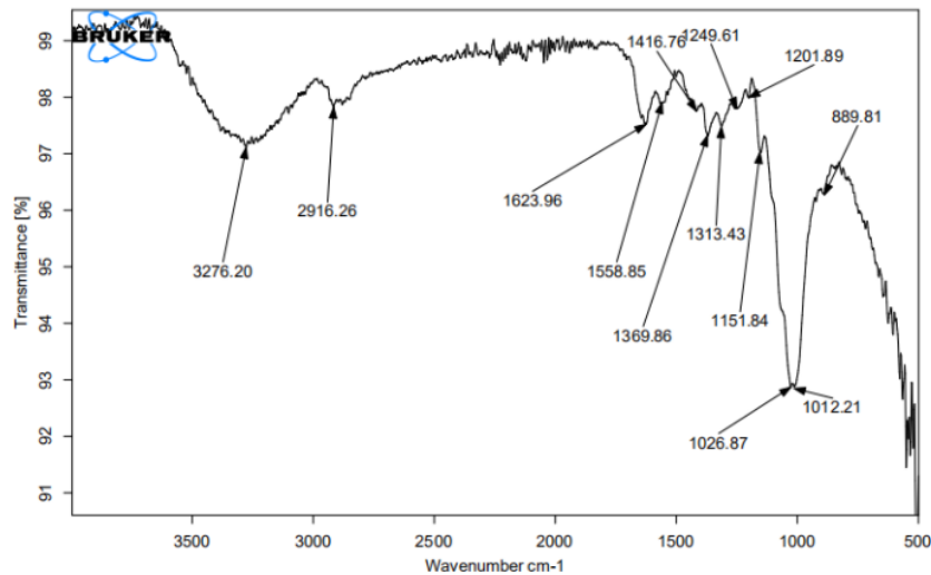
Gambar 4.2 Spektrum FTIR Nanokitosan
