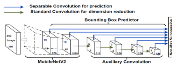
Gambar 2.5 Architecture Of SSD Lite [9].
