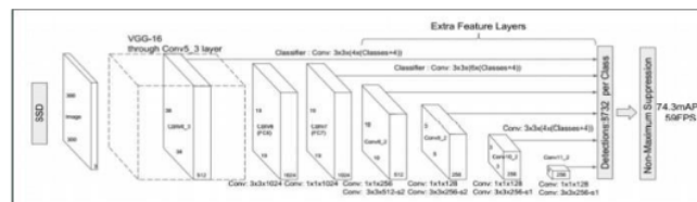
Gambar 2.4 Arsitektur Single Shot Detector
