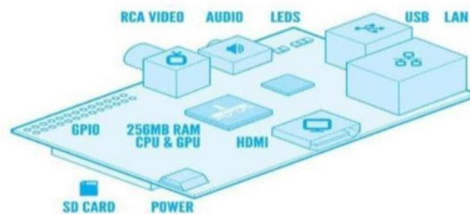
Gambar 2.1 Komponen Raspberry Pi Model B+
