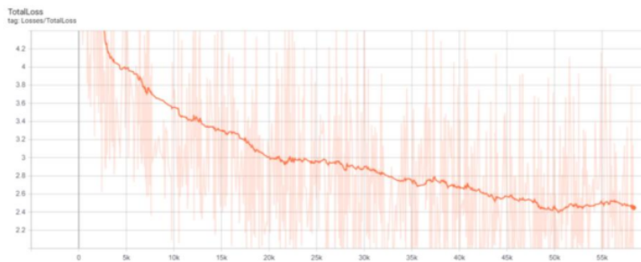
Gambar 4.7 Grafik Total Loss
