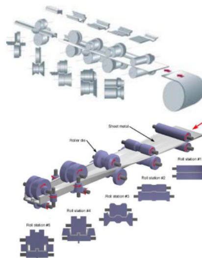
Figure 1. Roll Plate Processing [1]
