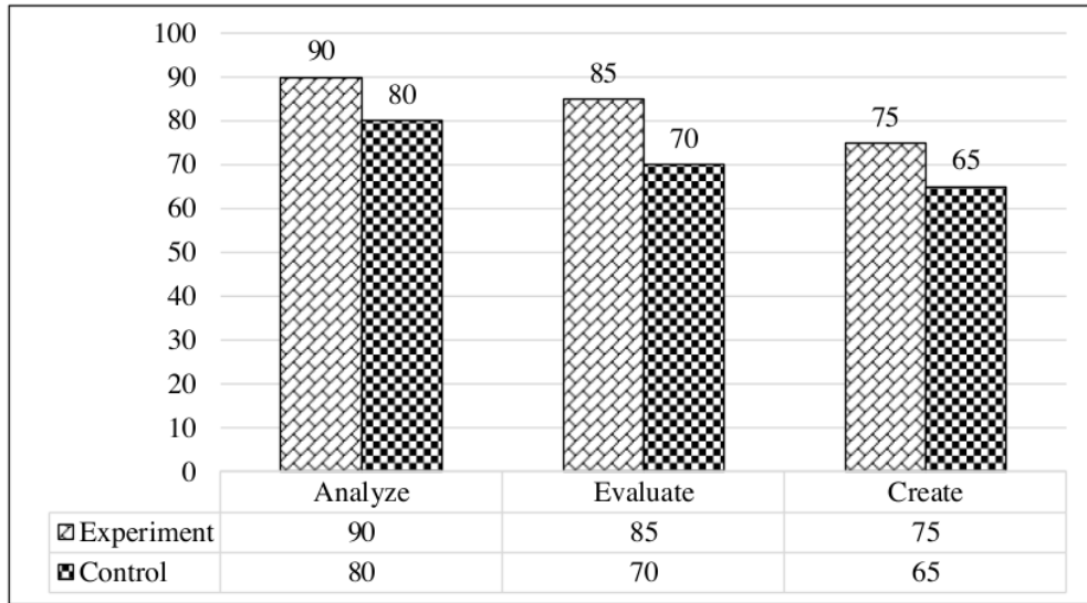
Figure 3. Posttest Data
