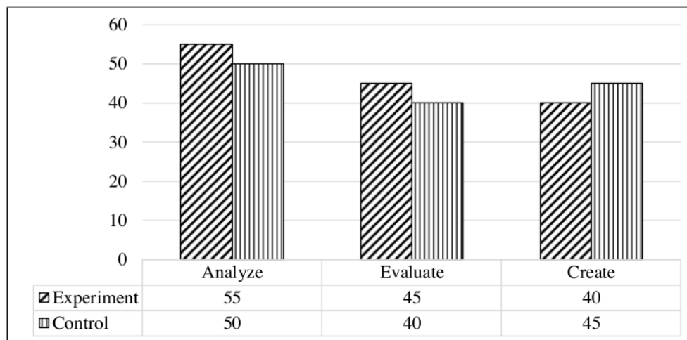
Figure 2. Pretest Data
