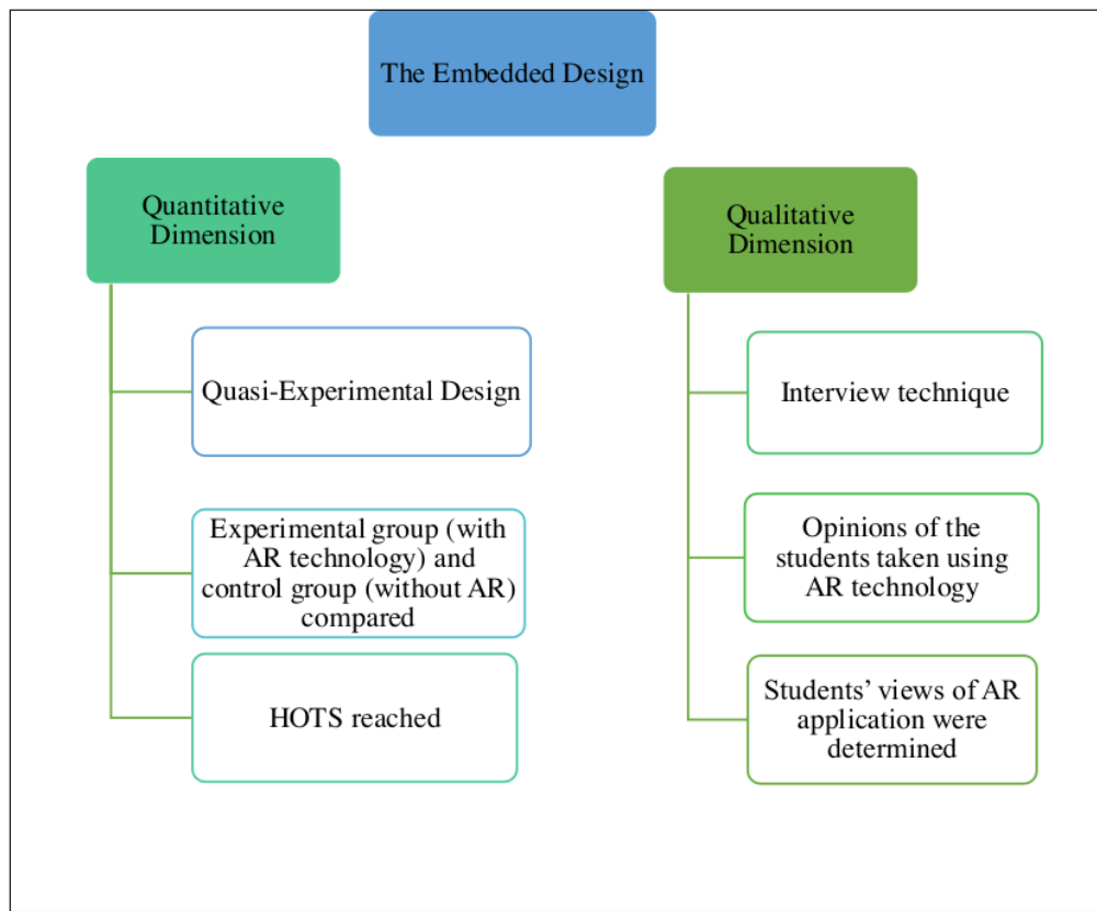
Figure 1. Research Method
