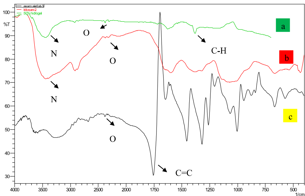
Fig. 6: FTIR Spectra of (a) Chitosan-graft-poly (acrylic acid) superabsorbent hydrogel, (b) Chitosan, (c) Acrylic Acid
