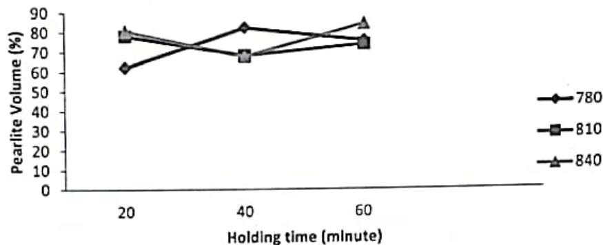
Figure 4.11 The influence of holding time toward pearlite volume at each temperature
