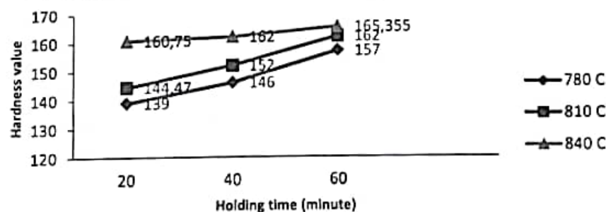
Figure 4.1 Chart between hardness value and holding time
