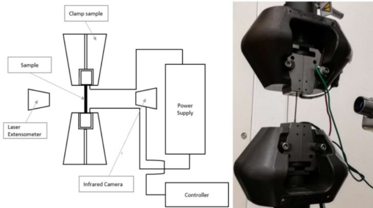
(a). Schematic of resistance heating system (b). Photo of clamp used to hold sample Figure 1. Configuration of tensile test equipment with resistance heating (RH).
