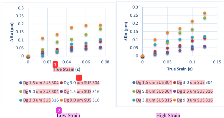
Figure 6. The increase in surface roughness in various Dg of SUS 304 and SUS 316 TMF.
