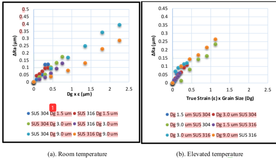
Figure 8. Relationship between increase in surface roughness ( \Delta R_a ) production of grain size ( D_g ) and true strain ( \epsilon ).
