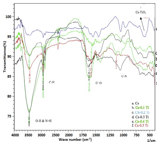
Fig. 1. FTIR pattern of chitosan bioplastic and chitosan- \text{TiO}_2 nanocomposites
