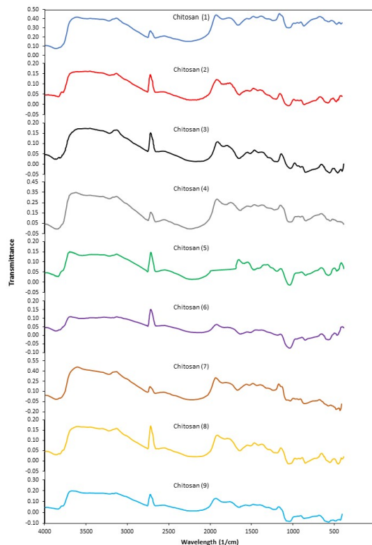
Fig. 2: FTIR spectra of treated shrimp shells
