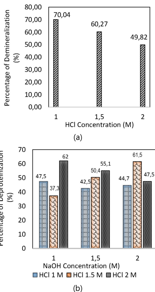
Fig. 1: Effect of different chemical concentrations on the (a) percentage of demineralization, (b) percentage of deproteinization
