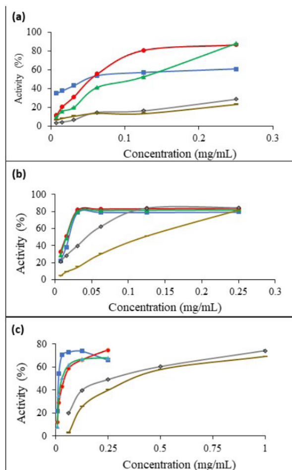
Figure 3. Antioxidant capacity of extracts based on the scavenging activities of (a) free radicals and (b) cation radicals, as well as (c) reducing power of ferric ions for (■) ascorbic acid, (●) the leaf extract of Centella asiatica , (▲) the leaf extract of Hydrocotyle verticillata , (◆) the pericladial petiole of C. asiatica and (▼) the pericladial petiole of H. verticillata .
