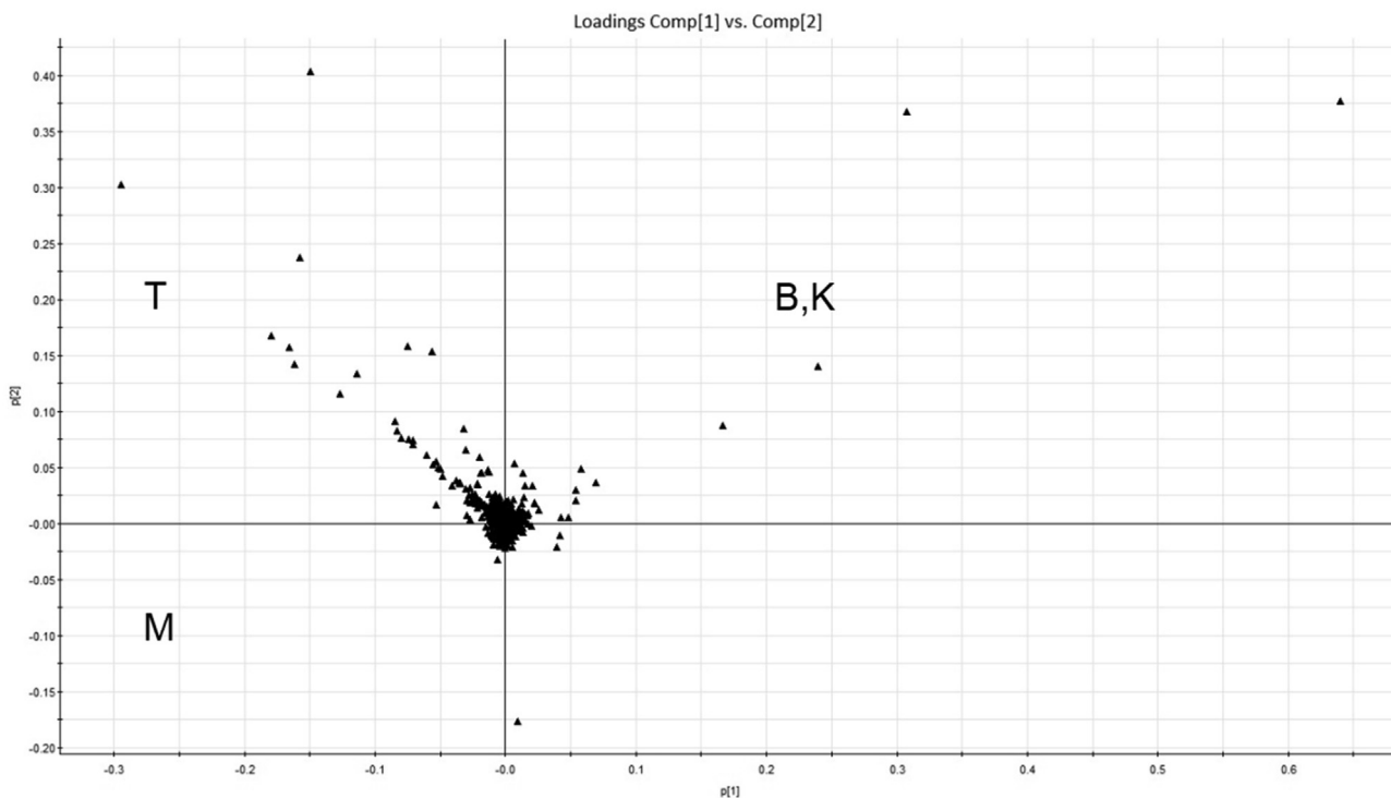
Figure 4. The PCA loadings plot for the four RJ samples with each dot representing a m/z -RT variable. The selected variables (red box) are shown as compounds unique to sample T.
