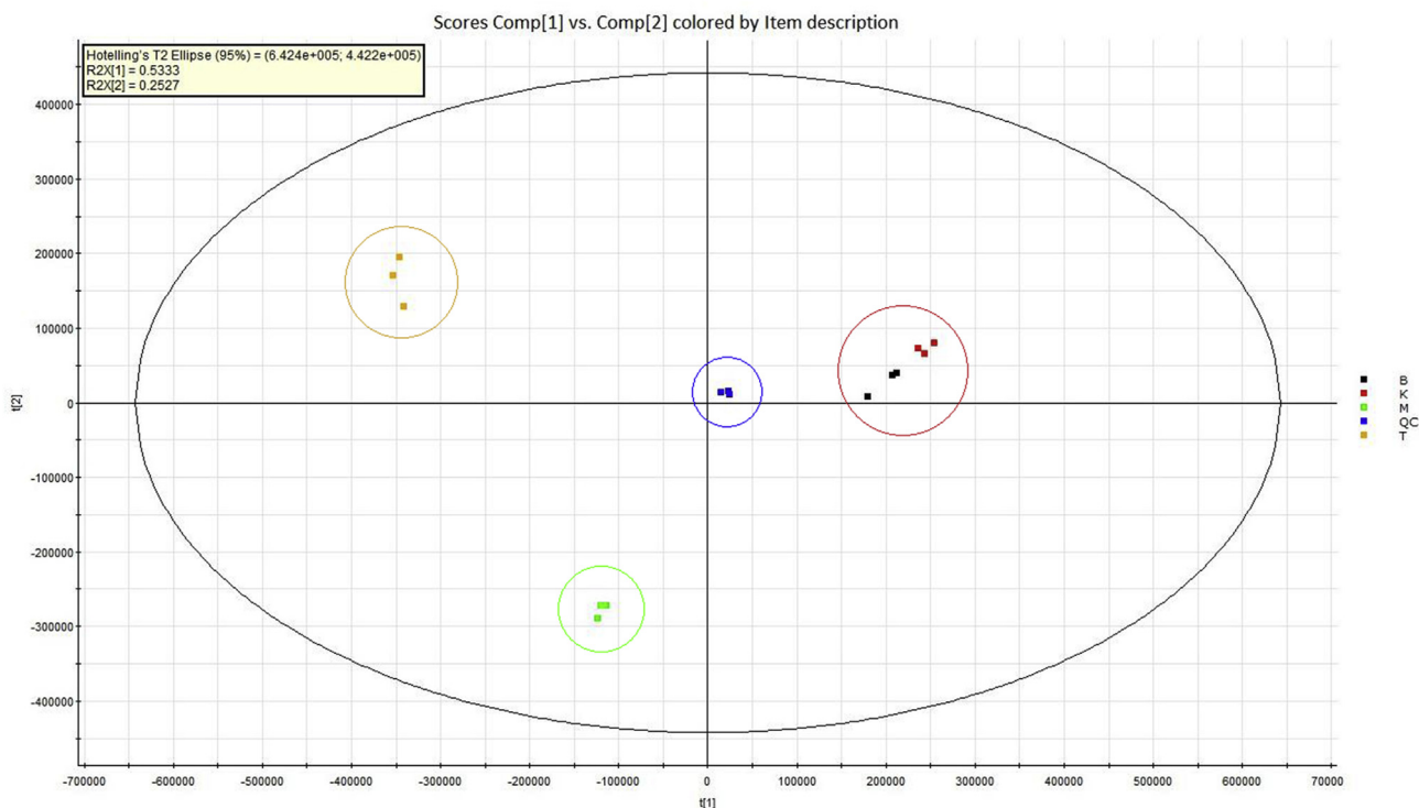
Figure 3. The PCA scores plot for the RJ samples. The first two principal components are shown. The ellipse represents the 95% confidence interval of the PCA model. Black: Banjarnegara (B), Red: Kediri (K), Green: Demak (M), and Orange: Tuban (T).
