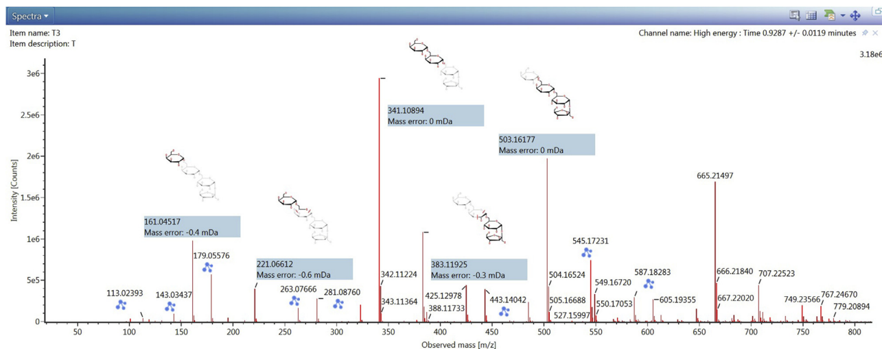
Figure 5. MSMS spectrum of stachyose, identified as one of the major marker constituents of royal jelly sample collected from Tuban (T), Indonesia.
