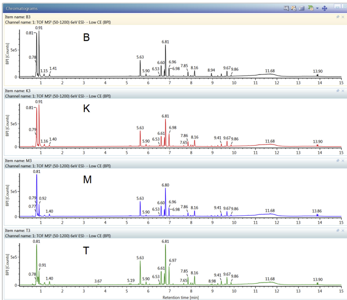
Figure 2. UPLC-QTOF/MS BPI chromatograms of four RJ samples from Banjarnegara (B), Kediri (K), Demak (M), and Tuban (T) in Indonesia.
