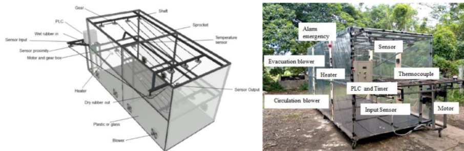
Fig. 3 Rubber dryer machine and components
