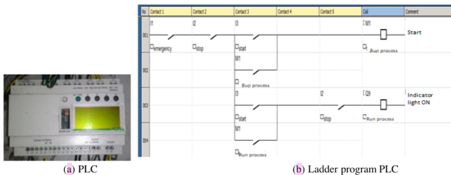
Fig. 2. PLC Zelio Smart Relay SR3B261FU
