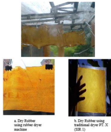
Fig. 11 Quality result testing of dry rubber
