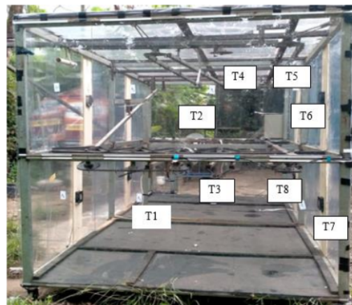
Fig. 5 Position sensor of temperature using thermocouple
