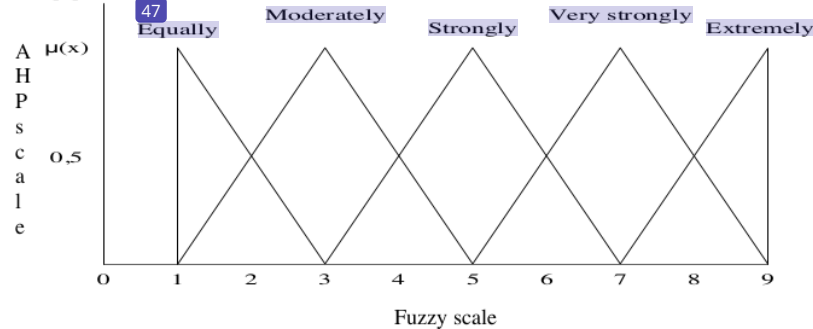
Figure 1. Membership function of fuzzy number.
