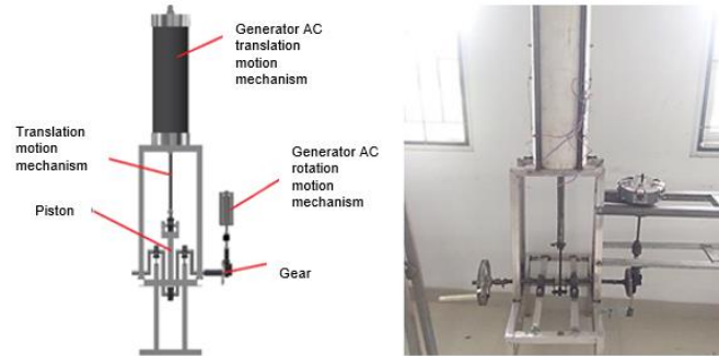
Fig 5. Generator AC with Translation and Rotation Mechanism
