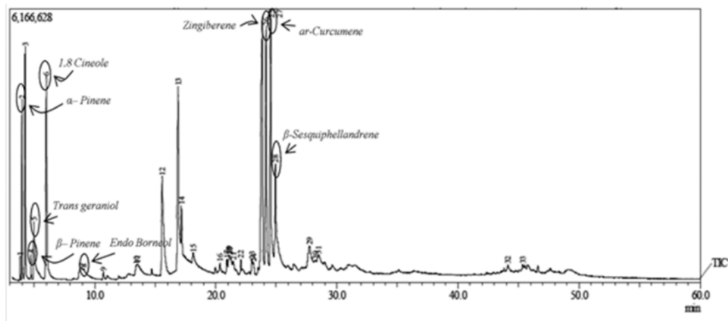
FIGURE 1. GC MS analysis of red ginger essential oil
