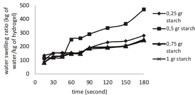
Figure 5. The relationship between the amount of starch and the water absorption properties of polymer starch-g-poly(potassium acrylate-co-acrylamide)
