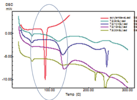
Figure 9. The result of DSC thermal poly (Potassium Acrylate-co-Acrylamide)
