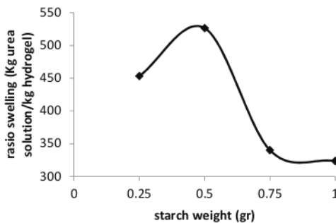
Figure 8. The relationship between the starch content and urea solution absorption of hydrogel
