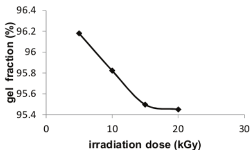
Figure 1. Effect of irradiation doses on gel fraction
