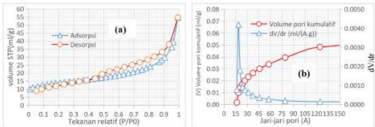
Gambar 4. Grafik analisis BET (Brunauer Emmet Teller), (a) Isoterm adsorpsi-desorpsi nitrogen, (b) Metode BJH desorpsi
