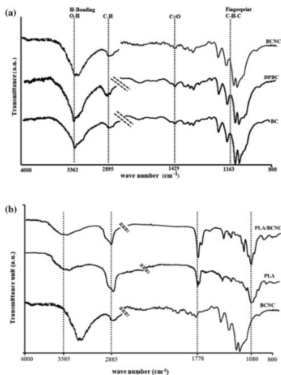
Figure 1. FTIR spectra of: (a) isolation of BCNC step (BC; D-BC; BCNC); (b) fabrication of biocomposite step (PLA; PLA/BCNC-5%).
