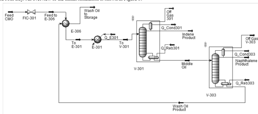
Figure 6. Simulation before feed splitting.
