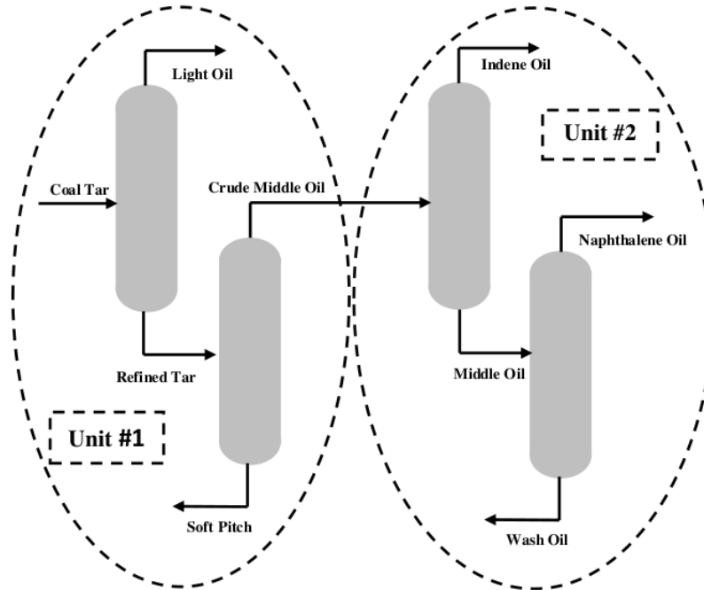
Figure 1. General description of coal tar distillation process.
