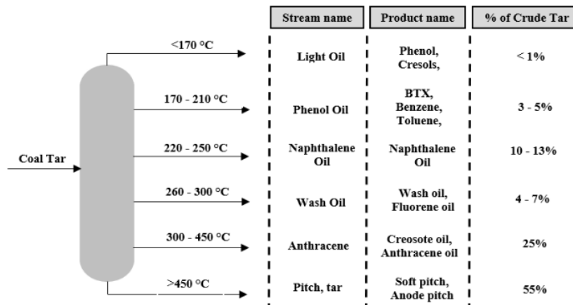
Figure 2. General composition of coal tar.
