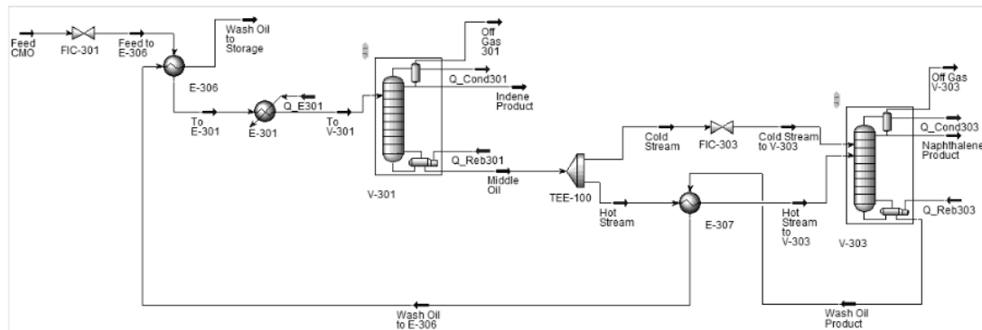
Figure 7. Simulation after feed splitting is applied.
