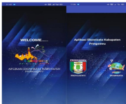
Figure 5. Splashscreen
