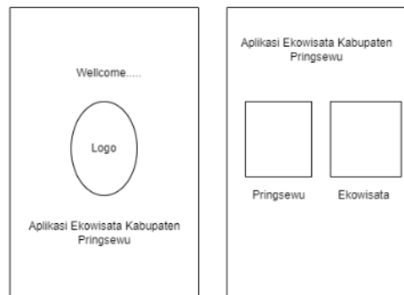
Figure 4. Splash Screen
