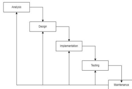
Figure 1. Waterfall Model
