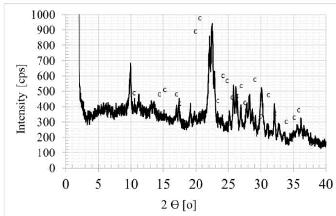
Fig. 3. The X-Ray diffraction (XRD) of natural zeolite.
