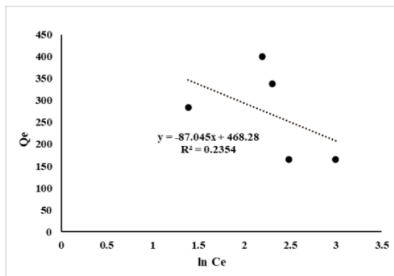
Fig. 6. Temkin isotherm model of natural zeolite 3000 \mu\text{m} .
