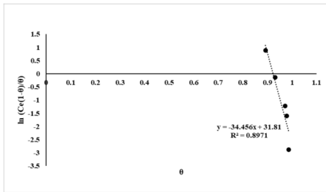
Fig. 8. Fowler-Guggenheim isotherm model of natural zeolite 3000 \mu\text{m} .
