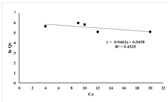
Fig. 9. Jovanovic isotherm model of natural zeolite 3000 \mu\text{m} .
