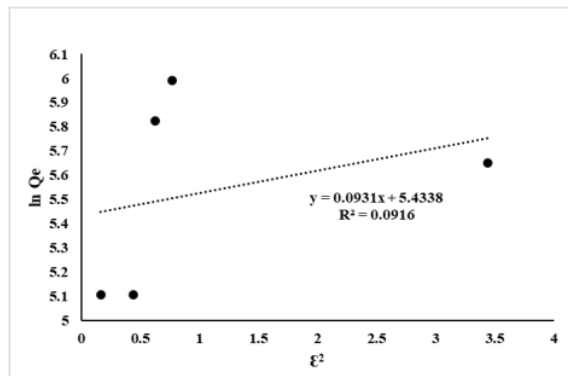
Fig. 7. Dubinin-Radushkevich isotherm model of natural zeolite 3000 \mu\text{m} .
