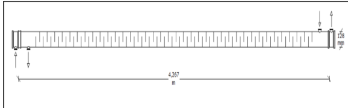
Fig. 2. Exchanger drawing.
