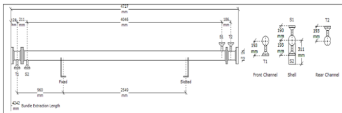
Fig. 3. Setting plan.
