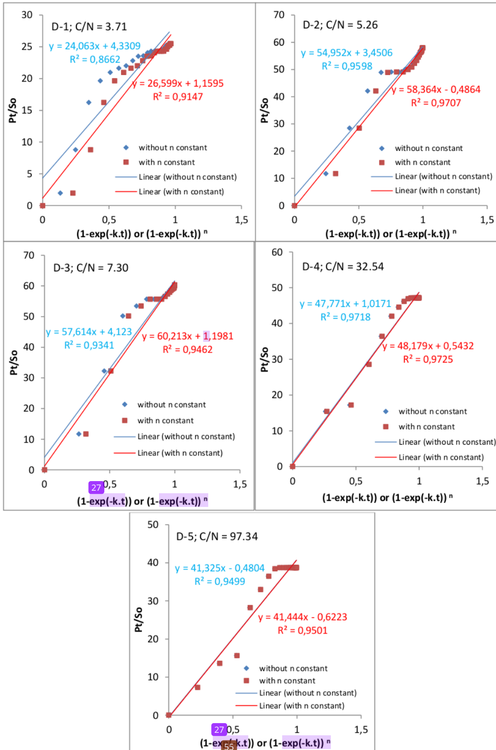
Fig 5. Comparison plotting 1-\exp(-k.t) and (1-\exp(-k.t))^n against Pt/So
