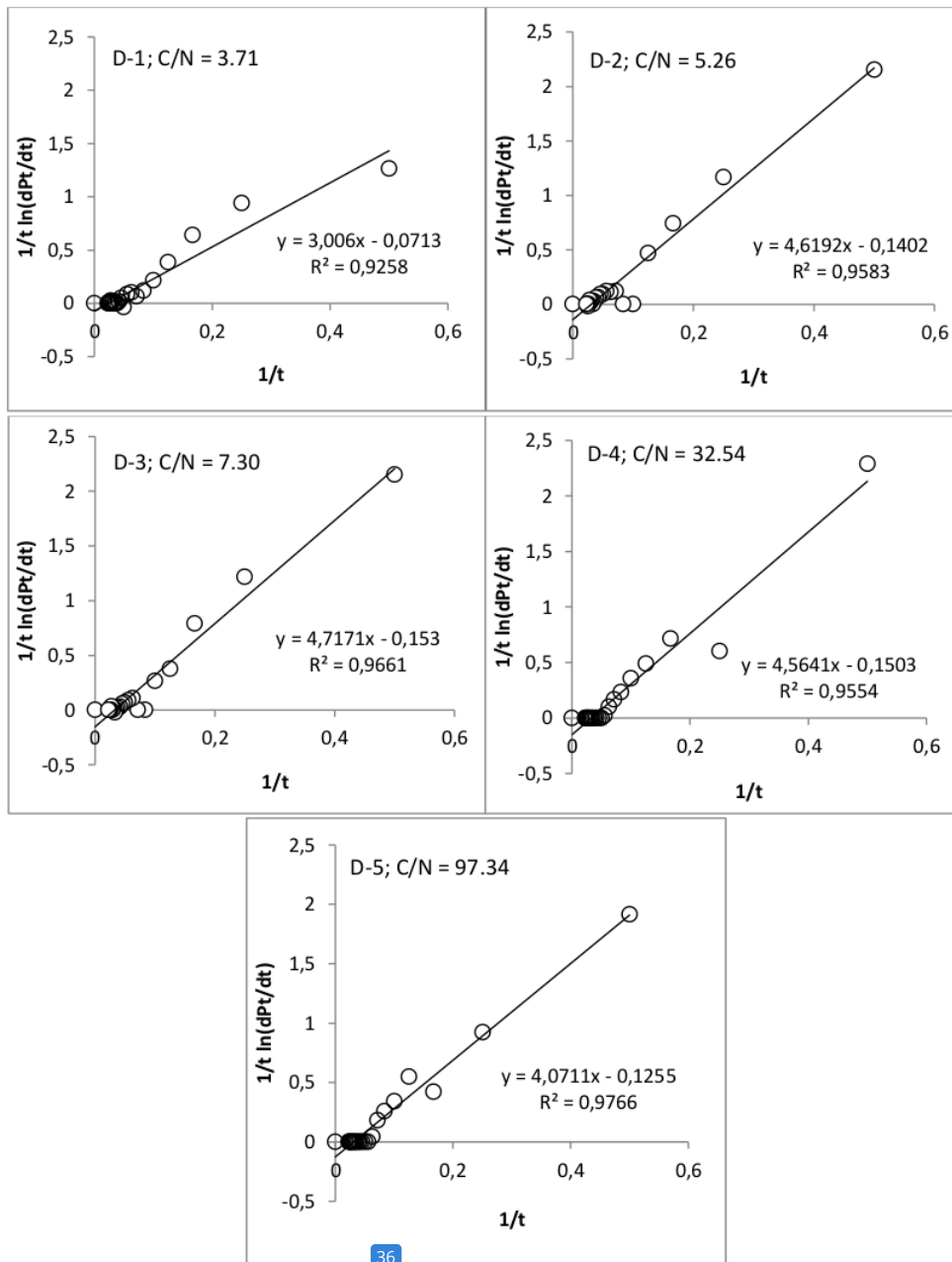
Fig. 4. Plot of 1/t (\ln(Pt/dt)) against 1/t
