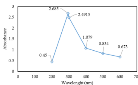
Figure 1. Absorbance value at various wavelengths using local POME liquid (dilution 10×).
