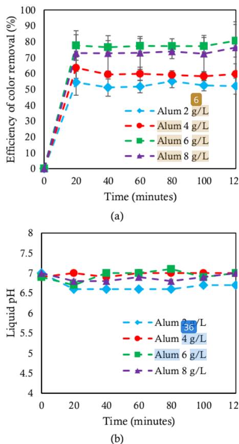
Figure 2. Effect of alum doses on the profiles of (A) color removal efficiency, (B) liquid pH.
