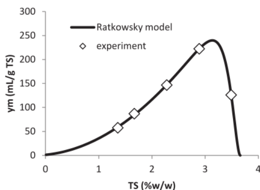
Fig. 4. Correlation between TS level on biogas yield based on Ratkowsky Model.
