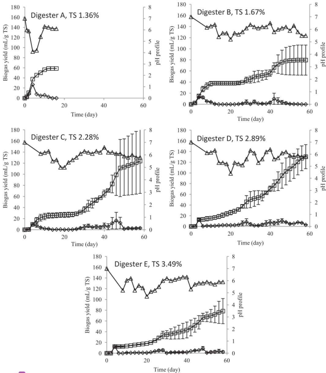
9 Fig. 1. The effect of total solid concentration on biogas production daily ( \diamond ), biogas production cumulative ( \square ), pH profile ( \Delta ).
