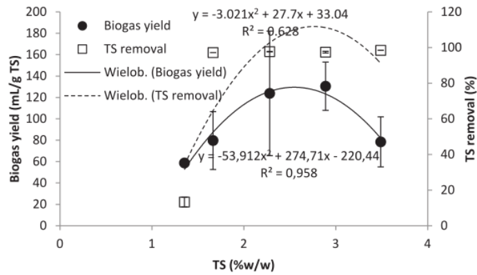
Fig. 2. Correlation between TS level on biogas yield and TS removal.
