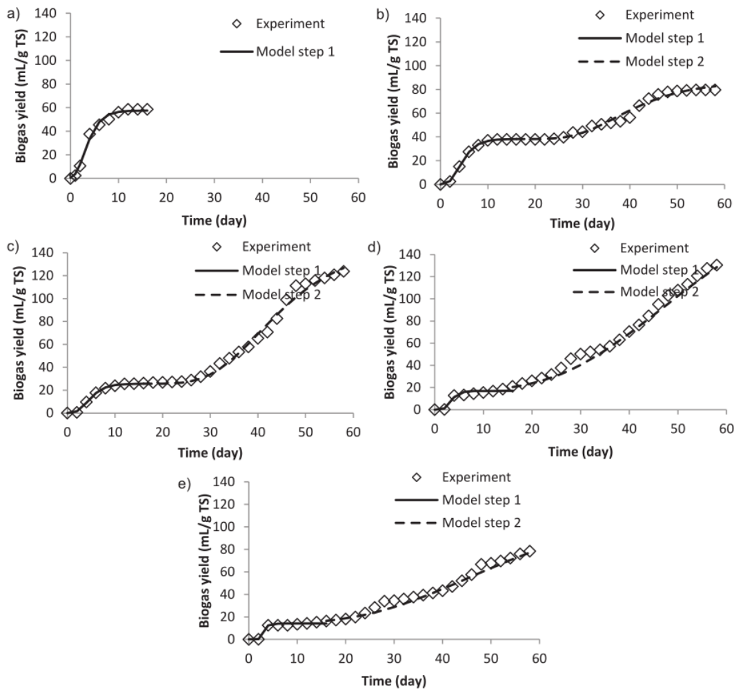
Fig. 3. Plot model step 1 and step 2 in digester (A) TS 1.36% w/w, (B) TS 1.67% w/w, (C) TS 2.28% w/w, (D) TS 2.89% w/w, (E) TS 3.49% w/w.
