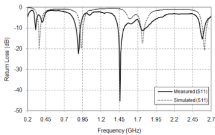
13 Fig 7. Simulated and measured result of return loss of multiband slot and array 1x2 antenna
