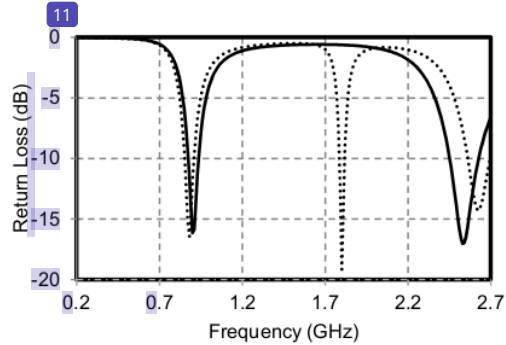
Fig 2. Return loss of multiband microstrip antenna using slot method.
