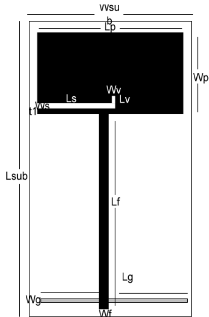
Fig 1. Microstrip antenna using slot method
