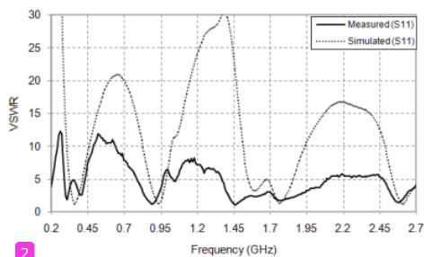
2 Fig 8. Simulated and measured result of VSWR of multiband slot and array 1x2 antenna
