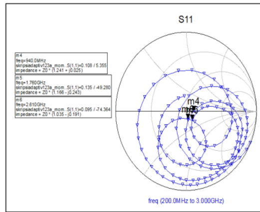
Fig 9. Input Impedance of Multiband Antenna
