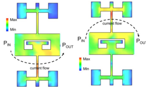
Fig. 10. Surface current distribution on of (a) lower band UWB-NotchBPF and (b) upper band UWB-Notch BPF.
