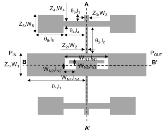
8 Fig. 1. The proposed UWB-BPF based on Crossed Dumbbell-Stub
