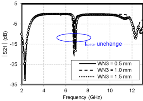
Fig 4. S_{21} (dB) response with varied W_{N3}
