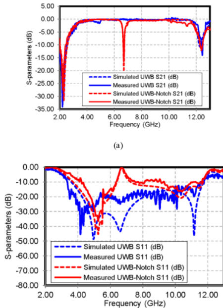
Figs. 9. Comparison of imulation and measurement results of (a) S_{21} , and (b) S_{11}
