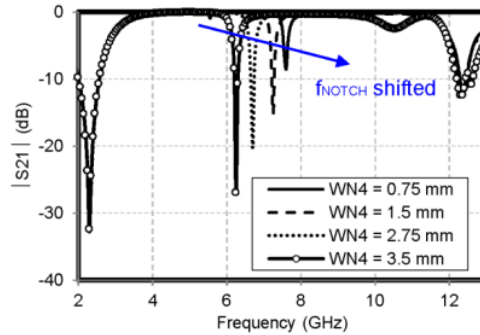
Fig 6. S_{21} (dB) response with varied W_{N4}
