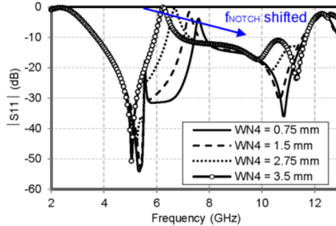
Fig 7. S_{11} (dB) response with varied W_{N4}
