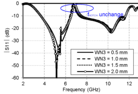
Fig 5. S_{11} (dB) response with varied W_{N3}
