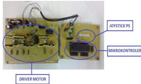
Figure 11. Main controller board dan motor driver
