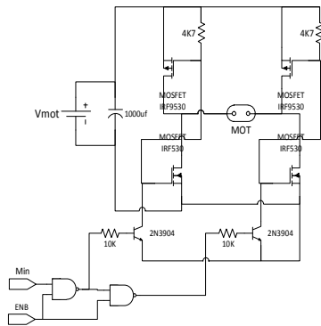
Figure 9. Mosfet H-bridge motor driver circuit diagram
