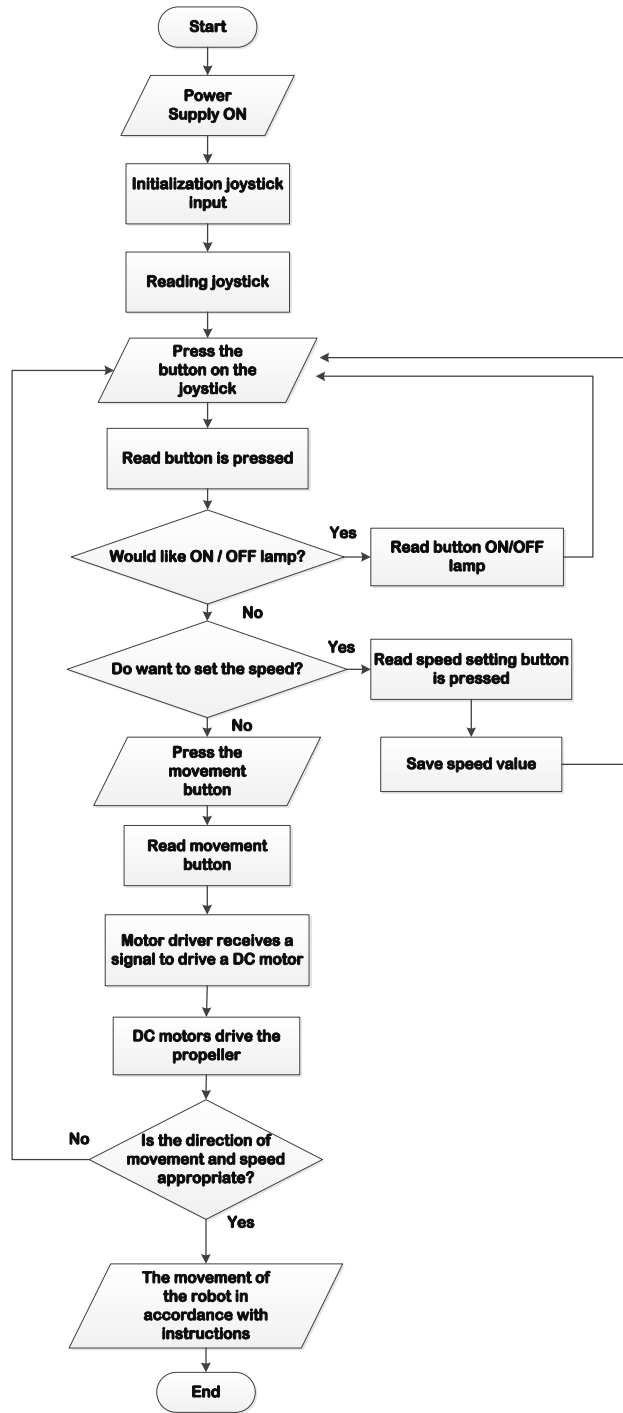
Figure 17. ROV system flowchart
