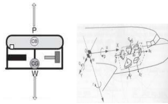
Figure 4. COG-COB Orientation on Vehicle [12-13]
