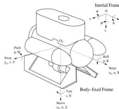
Figure 2. Vehicle degree of freedom [13]
